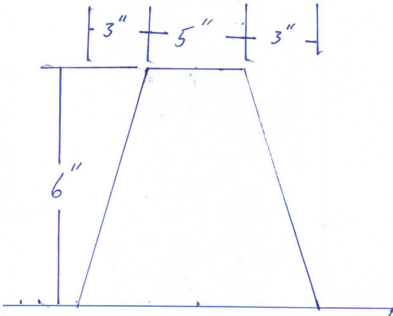
Extruded Asphalt Curb Detail
